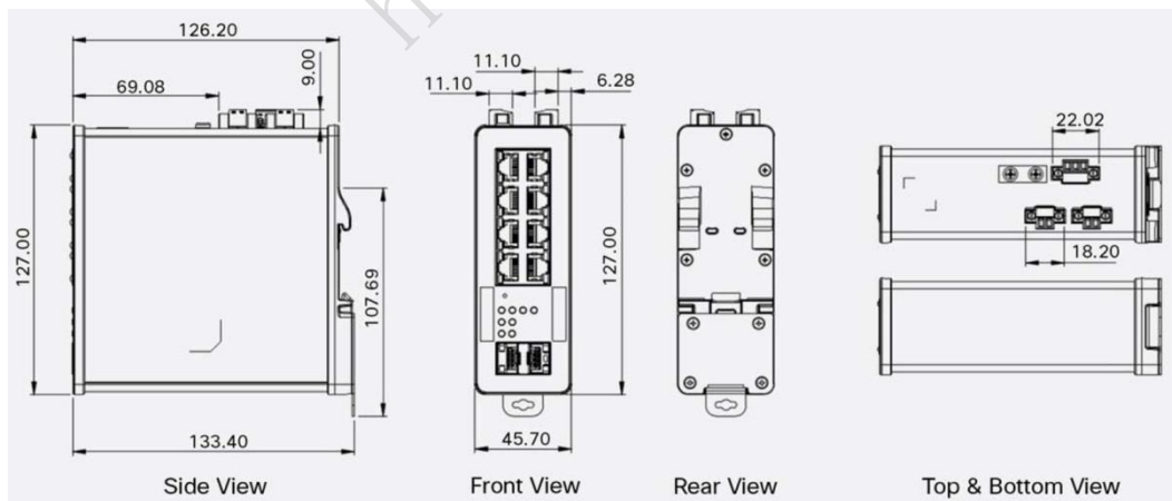
Figure 5. IE1000-8P2S-LM
